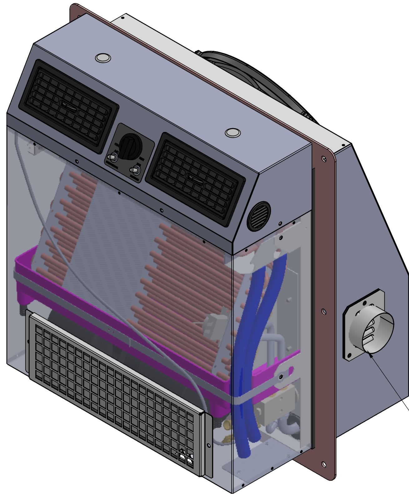
VIEW SHOWING INSIDE EVAPORATOR
