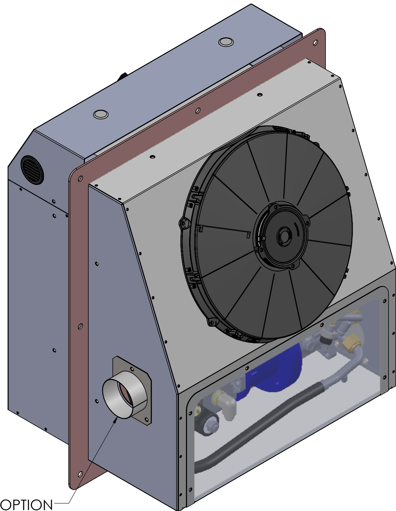
VIEW SHOWING INSIDE CONDENSER
