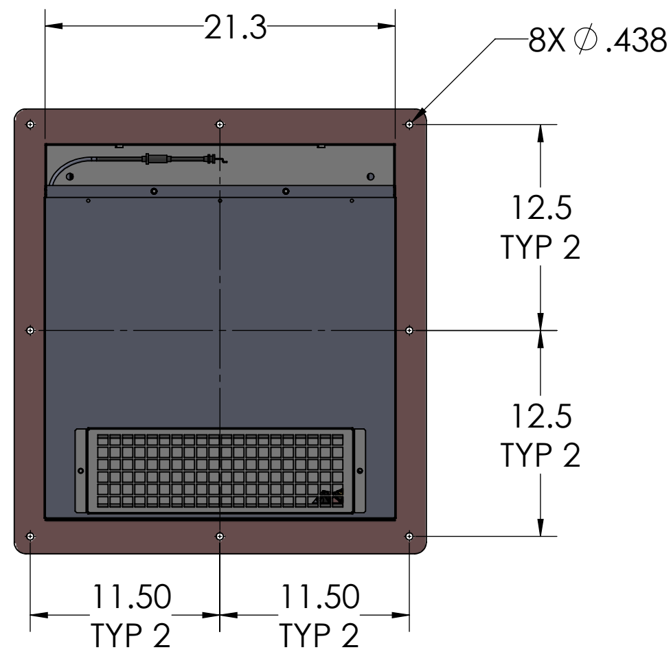
VIEW SHOWING WALL CUTOUT
