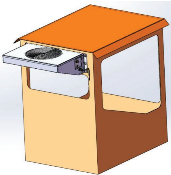
WALL MOUNTING
