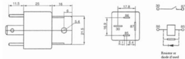
(TYPICAL RELAY)
